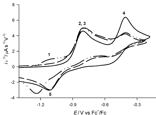
Figure 1. Cyclic voltammograms of 2 mM solutions of Zn- \text{Cp}_2\text{TiCl}_2 (—), Mn- \text{Cp}_2\text{TiCl}_2 (---), and Al- \text{Cp}_2\text{TiCl}_2 (- · - ·) recorded at a sweep rate of 0.1 V s -1 in 0.2 M Bu 4 NPF 6 /THF.
